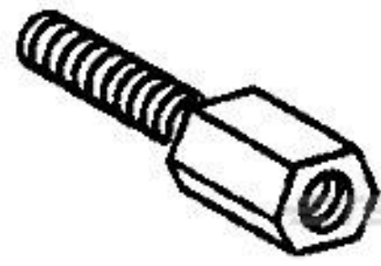
TE Part #5207953-3 FEMALE SCREWLOCK, SHORT, ZN
