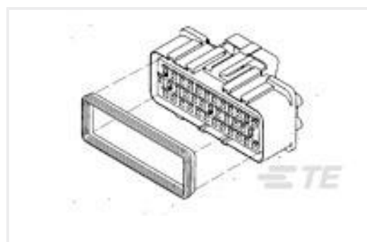
TE Part #346189-5 36 WAY REC HSG ASSY RED 60P P
