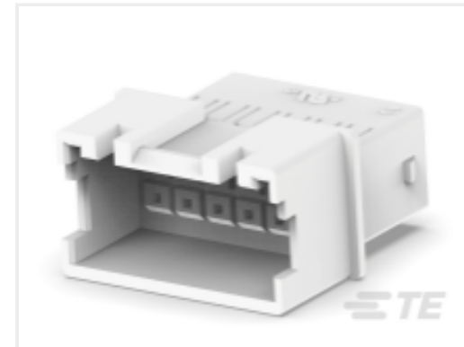
TE Part #1-2324201-2 HSG, REC, FREE-HANGING, GWT, DUALROW, EP2.5
