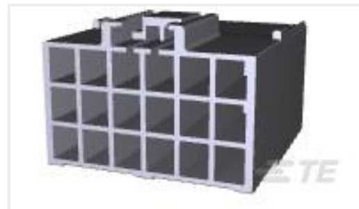
TE Part #176291-1 UNIV POWER CAP HSG 18P F/H
