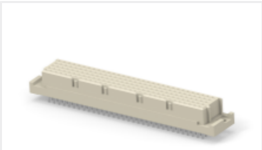
TE Part #284959-E STVE 160 F ABCDE VVVV 7-00 TL 4,0 * 137
