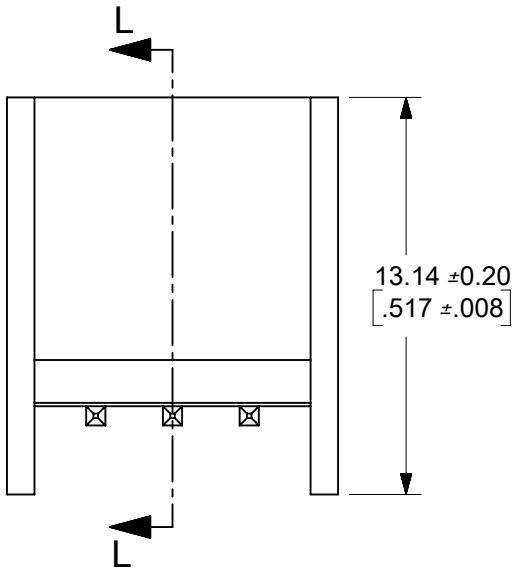
1 TO 6 CIRCUITS
