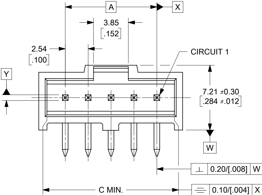
4 TO 32 CIRCUITS
