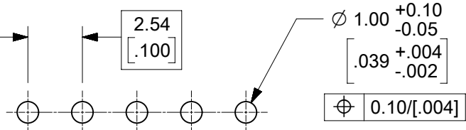
RECOMMENDED PCB PATTERN
