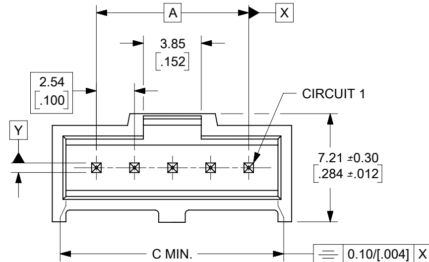
4 TO 32 CIRCUITS
