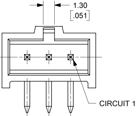
1 TO 3 CIRCUIT
