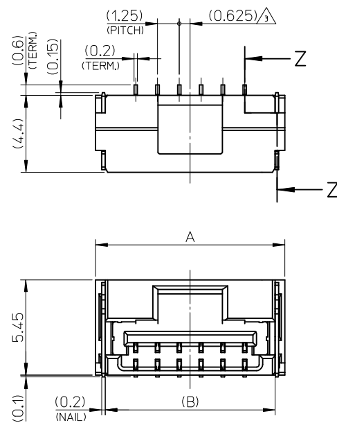
SECTION Z-Z
