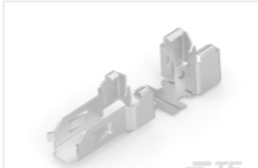
TE Part #1897796-2 REC SHIELD AR5 FOR RF S/L
