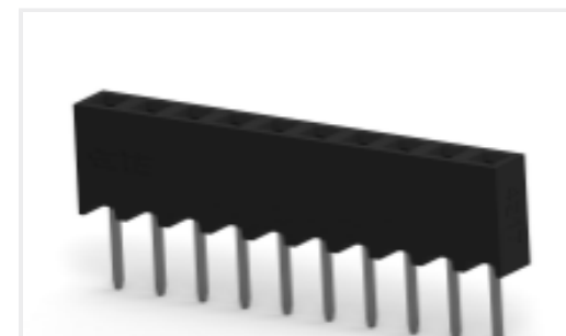
TE Part #1-2314878-0 10P,2MM,B-B,REC,SRVT,2.7,0.76AU,TB
