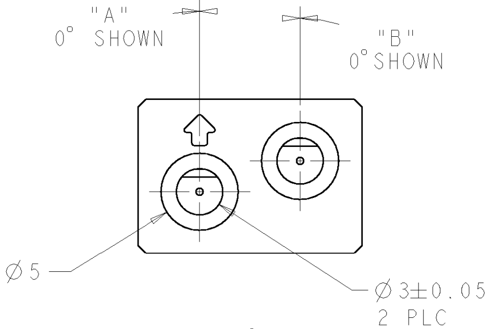
DETAIL C SCALE 4:1 1-1469267-1 SHOWN
