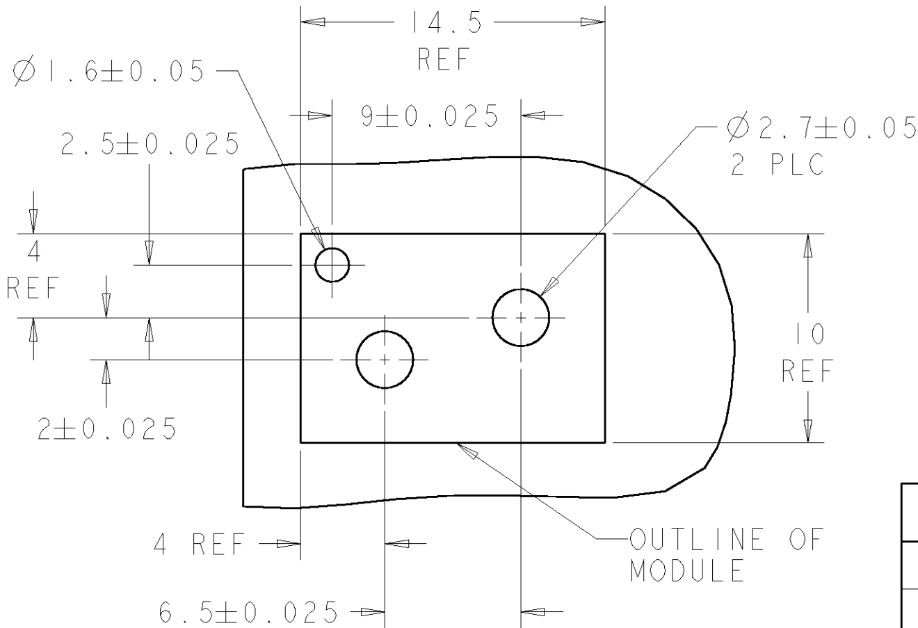
PCB LAYOUT
