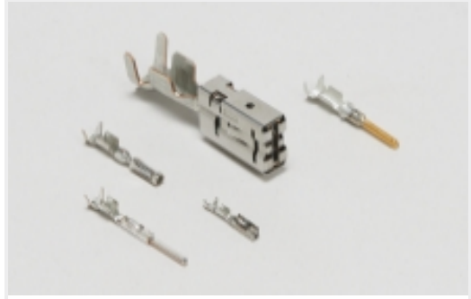
Automotive Terminals(53)
