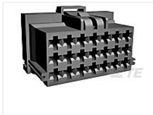
TE Part #8-968975-1 MCP2.8 GEH 21P
