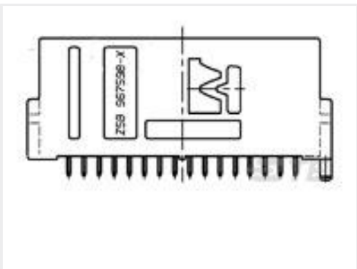
TE Part #967598-1 32pos MQS .63 header 180deg
