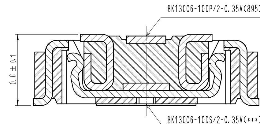
POWER CONTACT
