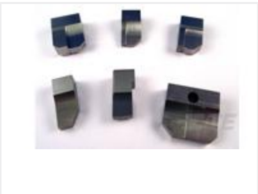
TE Part #6-854014-1 ANVIL, COMBINATION
