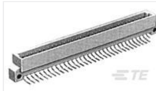
TE Part #5536052-5 ASSY,PIN,EUROCARD,TYPE B,LEAD-
