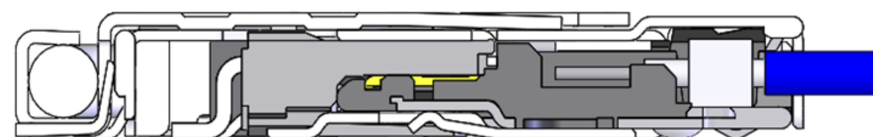
complete mating
