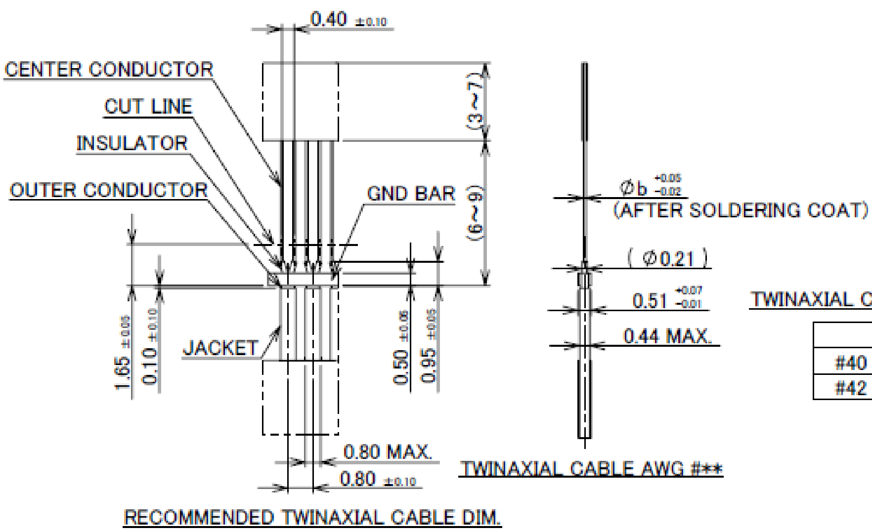
RECOMMENDED TWINAXIAL CABLE DIM.
