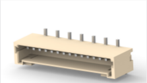
TE Part # 1-292371-5 SINGLE ROW POST HEADER ASS'Y SMT TYPE W/
