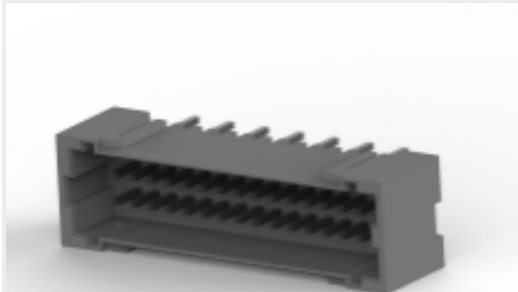
TE Part # 3-292208-0 MINI CT D/R DIP 30P V NAT
