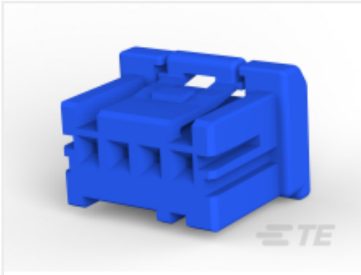
TE Part #2-1903390-3 GIC 2.5 W PLUG HSG 4P BLUE
