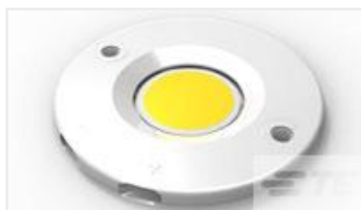
TE Part #2213254-1 LUMAWISE LED HOLDER Z50 LOW PROFILE 1919
