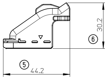
SHORT TYPE 560189-0101
