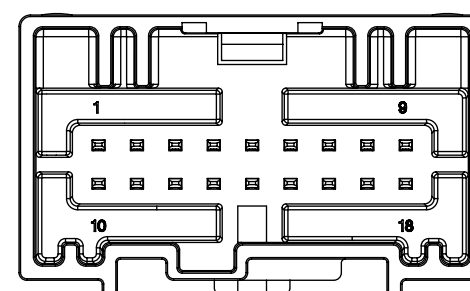
18 CIRCUIT
