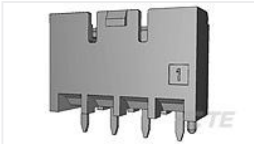
TE Part #1-1376382-2 5mm B-T-W Conn. 2P HDR ASSEMBL
