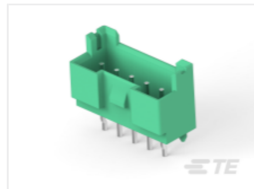
TE Part #8-2338245-5 EP2.5 HDR 5P VERT BOSS, GREEN, UL
