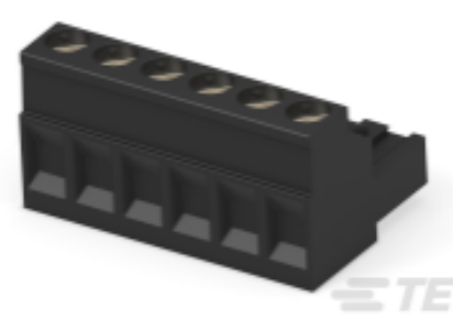
TE Part # 796635-6 6 POS 5.08MM R/A PLUG, TRM BLK
