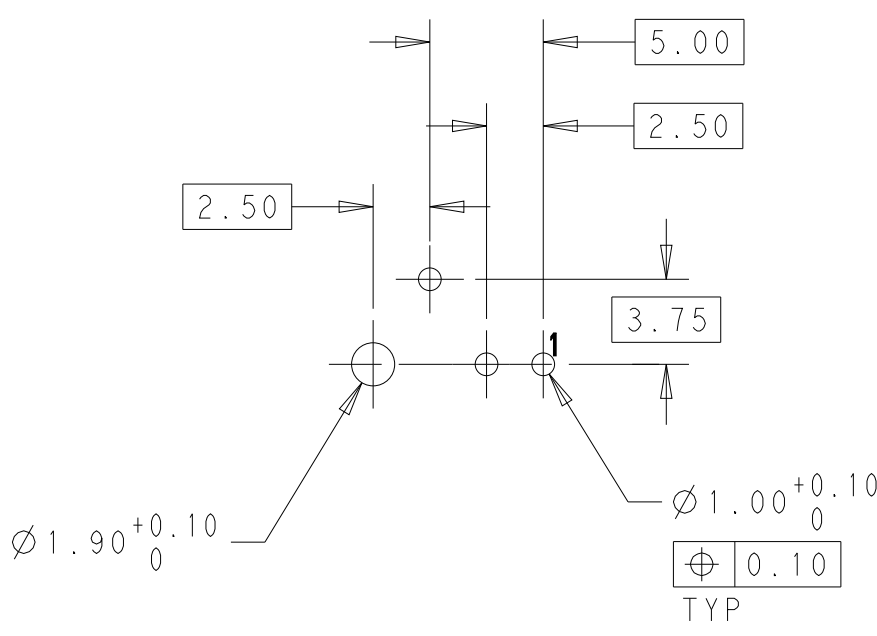
PCB LAYOUT D - SOLDER SIDE
