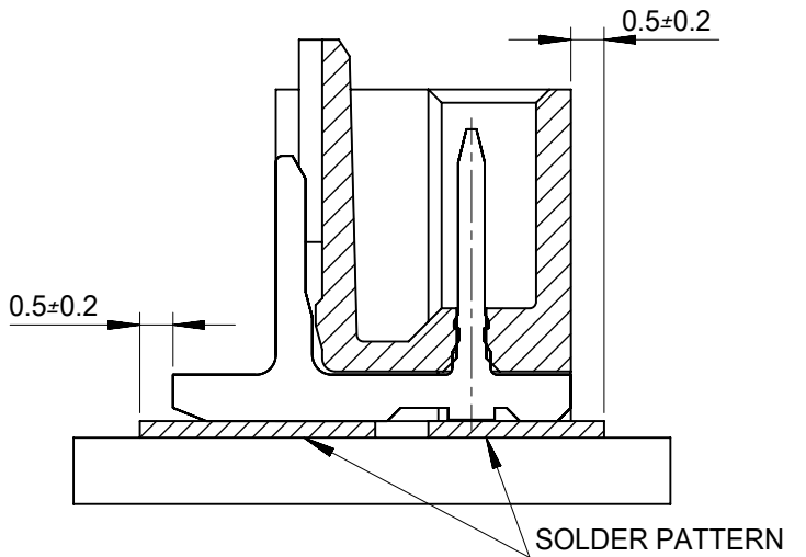
MOUNTING POSITION OF THE CONNECTOR
