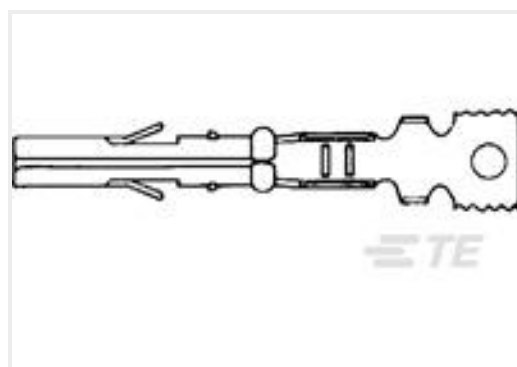
TE Part #641294-1 MR RECPT 26-18 PTPHBZ
