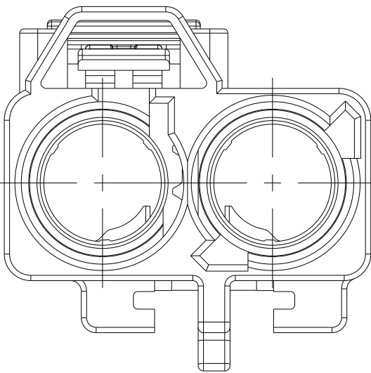
DETAIL N SCALE 4:1
