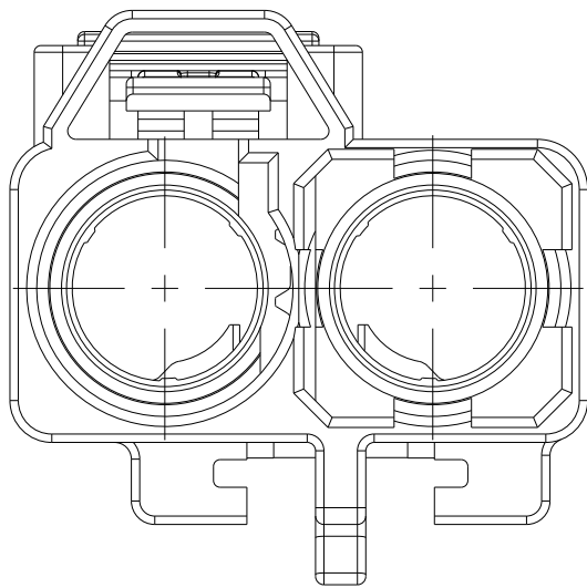
DETAIL Z SCALE 4:1
