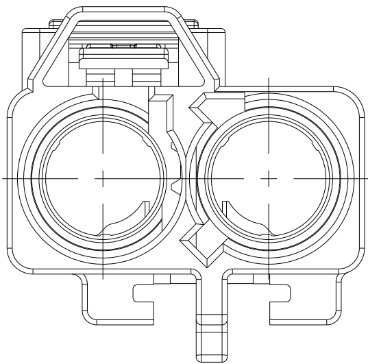
DETAIL F SCALE 4:1
