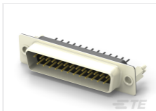
TE Part #2301835-1 AMPL PLUG HD20, VERT, 25P, B/L, 4-40 INS
