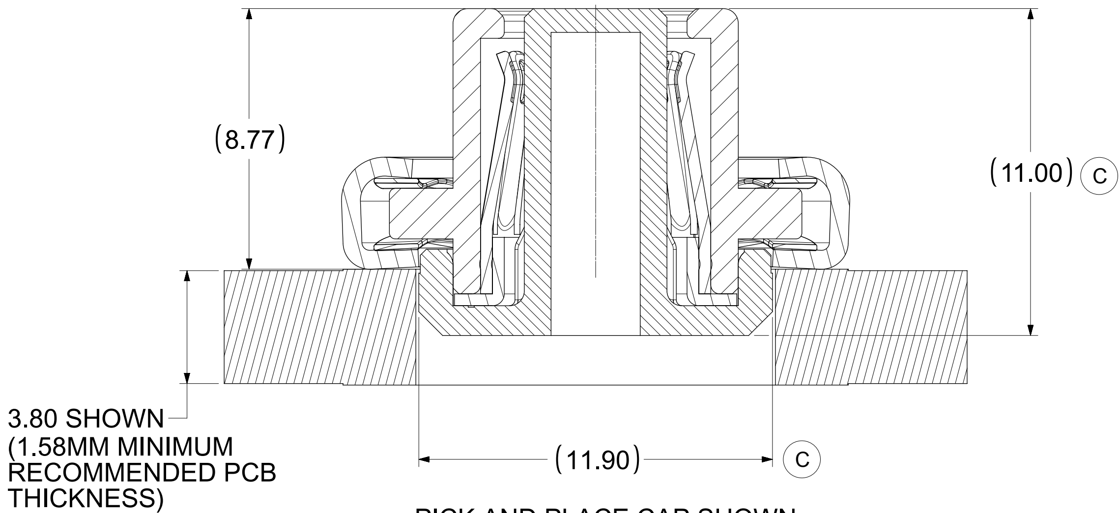
PICK AND PLACE CAP SHOWN
