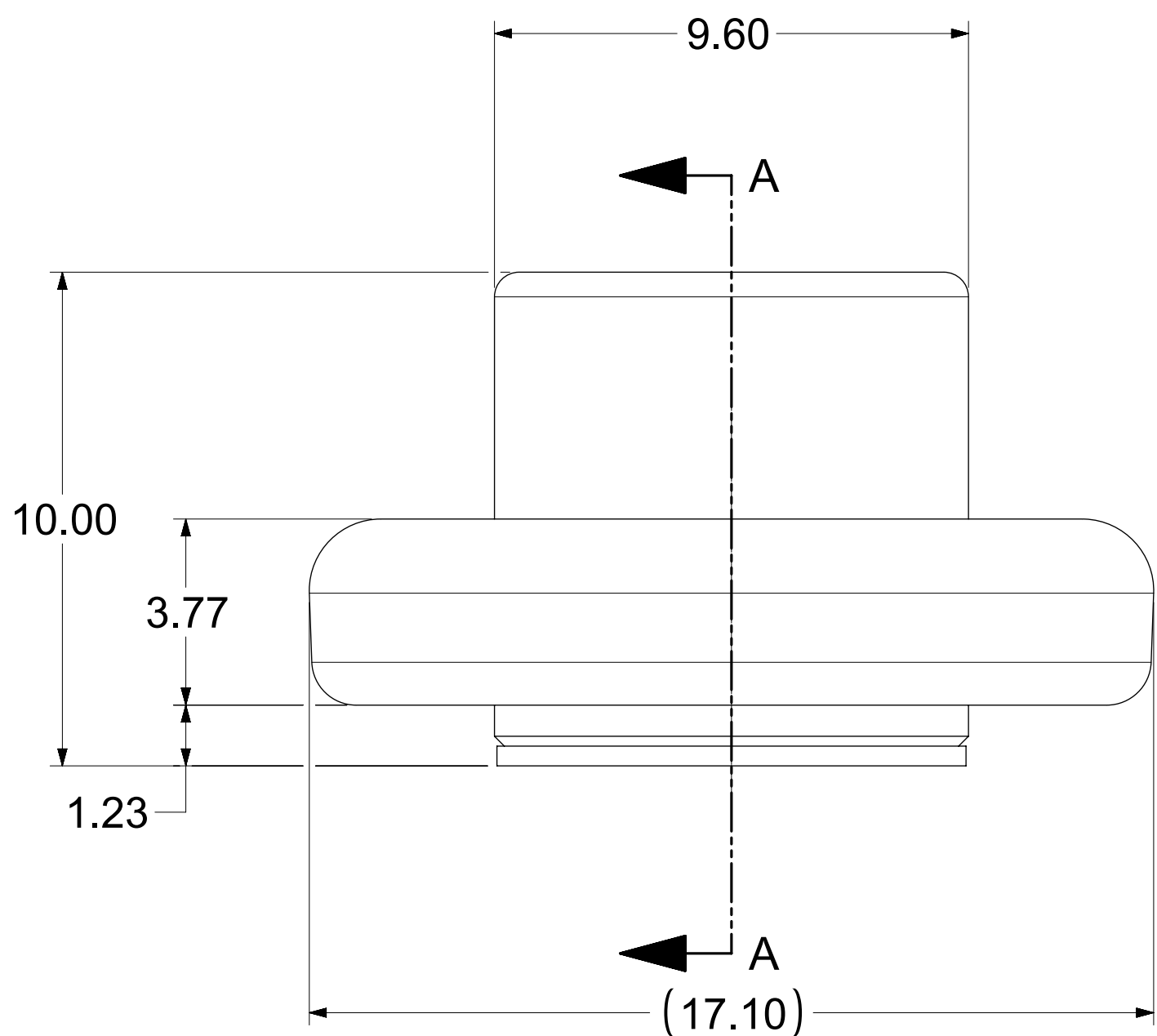
SOCKET ALONE (C)
