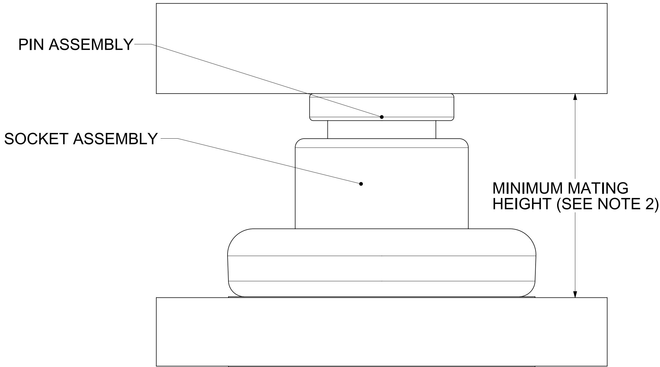
MATING PROFILE
