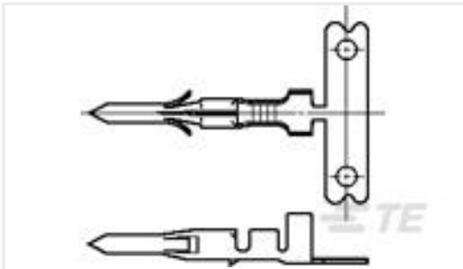
TE Part #350629-8 .062 COMM P&S PIN PRE TIN/PHBZ
