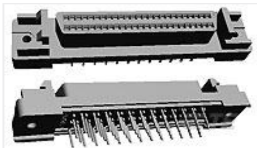
TE Part #5749069-1 20 50SR VERT RCPT ASSY
