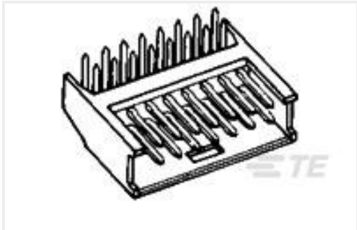
TE Part #280389-2 2X4P MODU II SHRD HDR,RT ANG, 0.38AU
