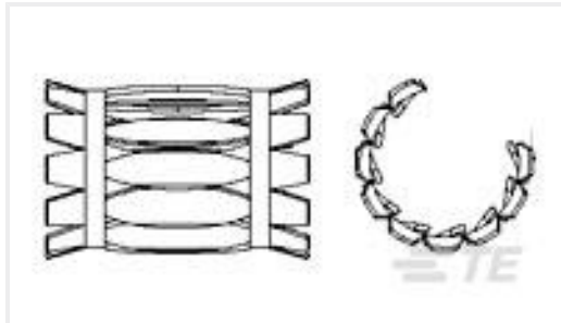
TE Part #7-192013-1 LA1A(.006)SIL
