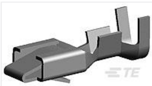
TE Part #640841-1 BLADE REC 250 20-16AWG BR
