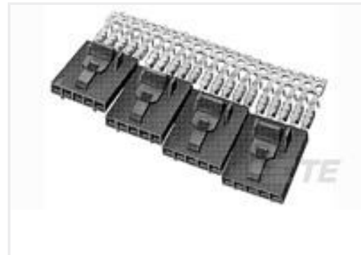
TE Part # 103960-5 4X6 MTE RCPT SR LATCH .100CL
