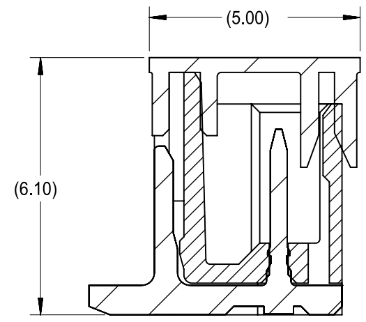
SECTION A-A (WITH CAP)
