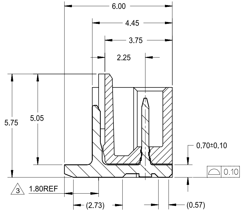
SECTION A-A (WITHOUT CAP)
