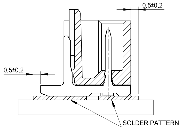
MOUNTING POSITION OF THE CONNECTOR
