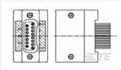
TE Part #3-1589488-1 STM025M5PQ = THRU-HOLE
