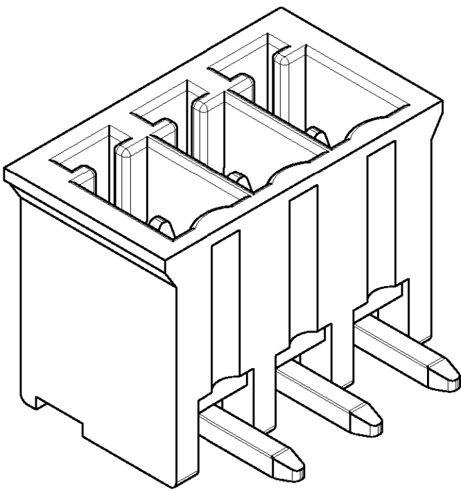
796695-3 AS SHOWN
