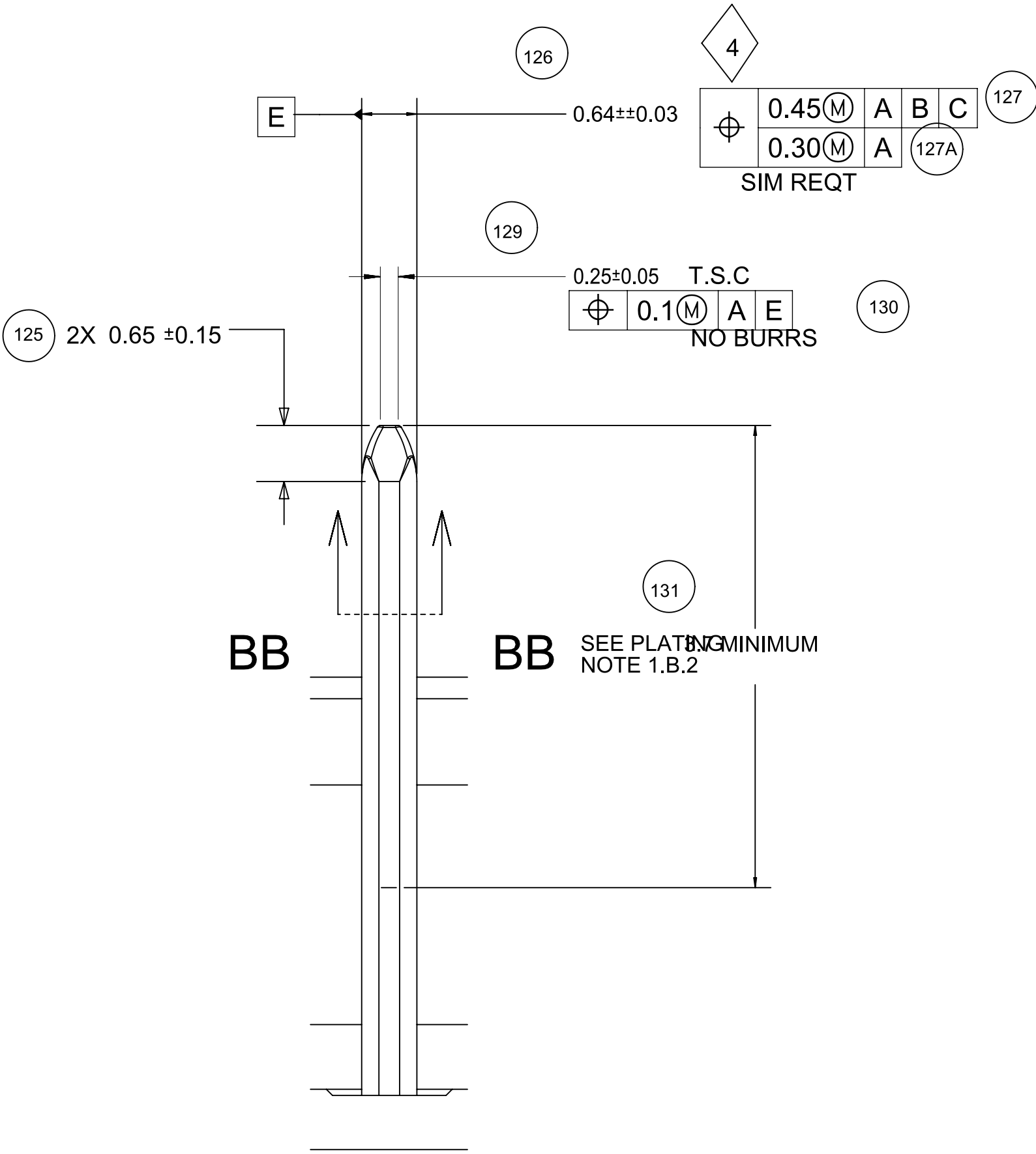
SECTION U-U TYPICAL
