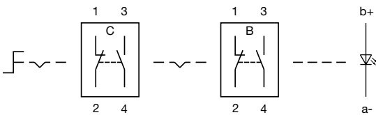
Wiring diagram 286
