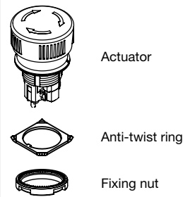
Each Part Number listed below includes all the black components shown in the 3D-drawing.
