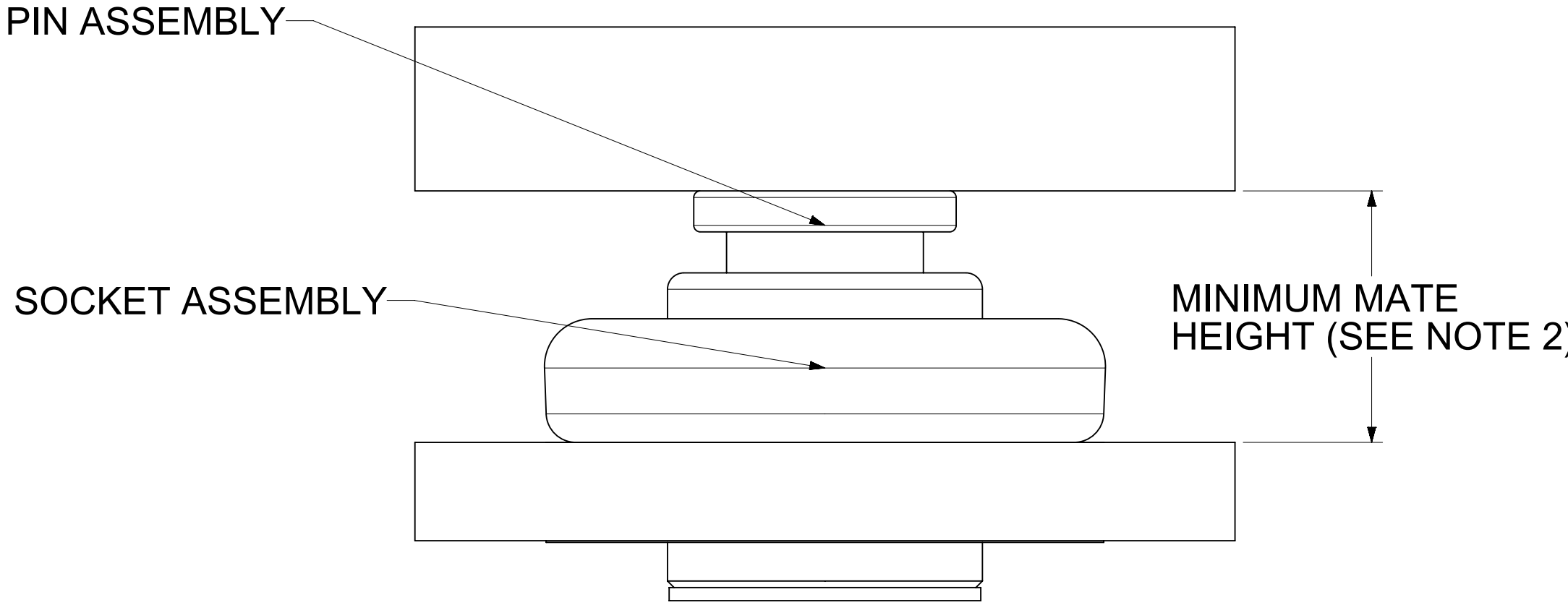
MATING PROFILE B3
