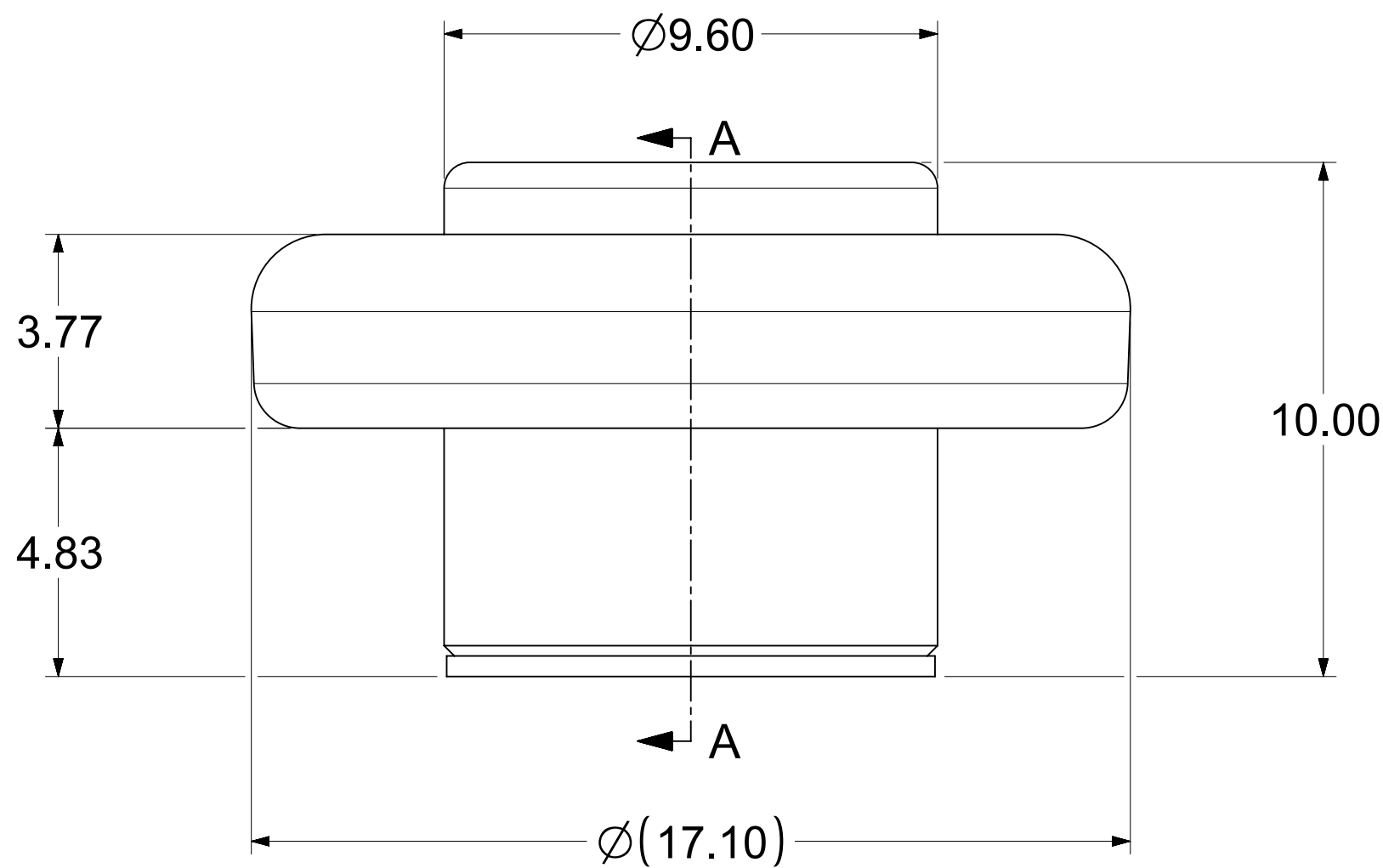
SOCKET ALONE
