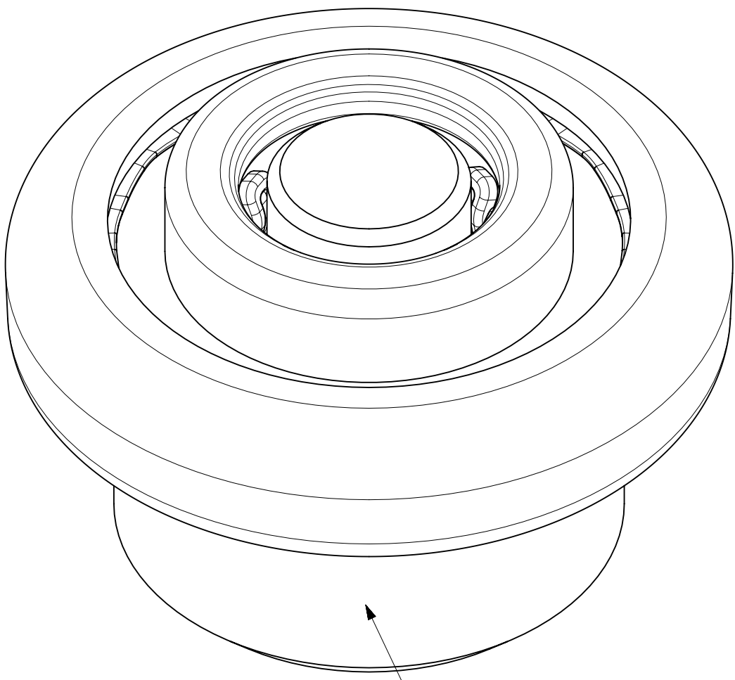
REMOVABLE PICK AND PLACE CAP SHOWN
