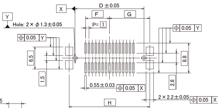
Recommended Land Pattern Diagram
