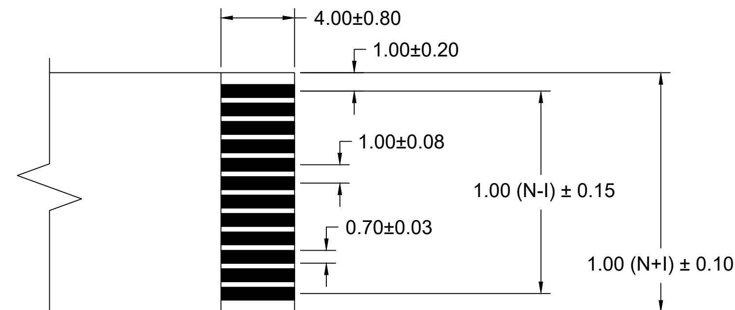
END TAIL DETAIL SCALE 5:1
