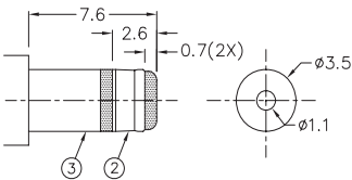
MATING PLUG
