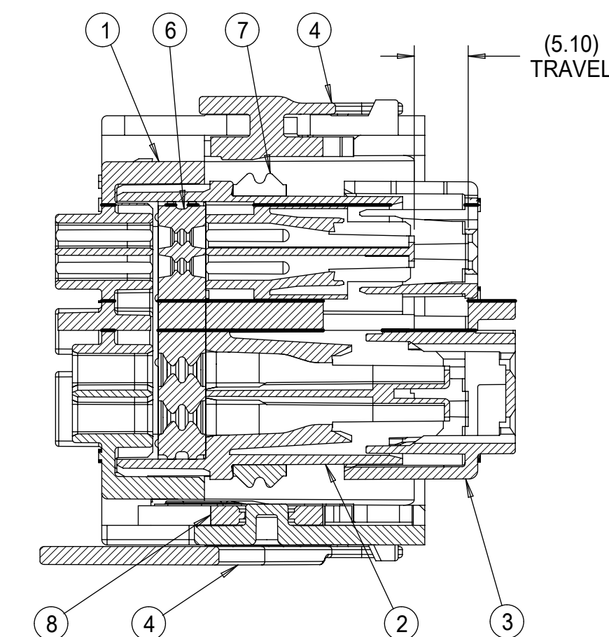
Section Y-Y
