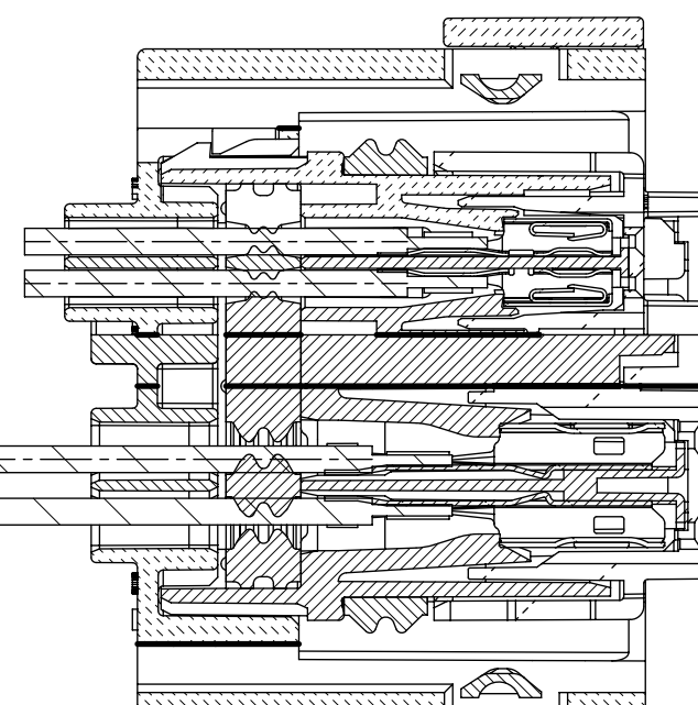
TERMINALS AND TPA SHOWN IN FINAL LOCKED POSITION Section X-X
