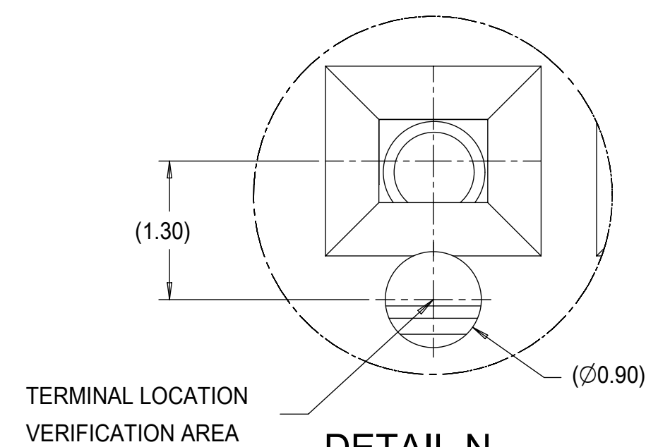
SCALE 20:1 0.64 TERMINAL LOCATION VERIFICATION HOLE
