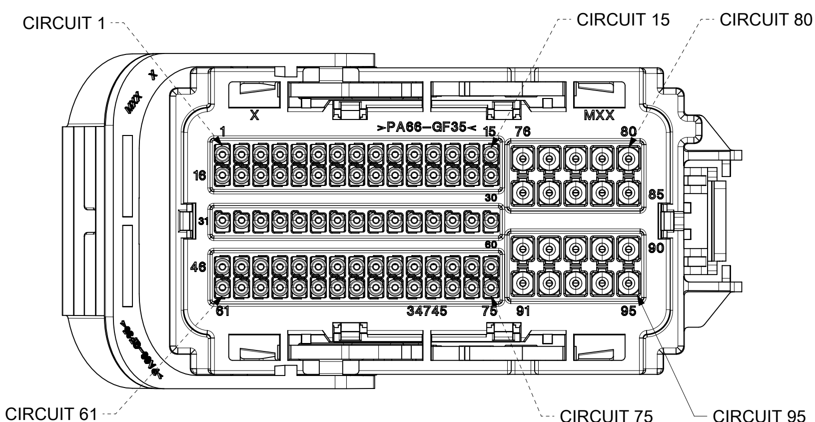
VIEW SHOWN WITH MOLEDED IN CAVITY PLUGS
