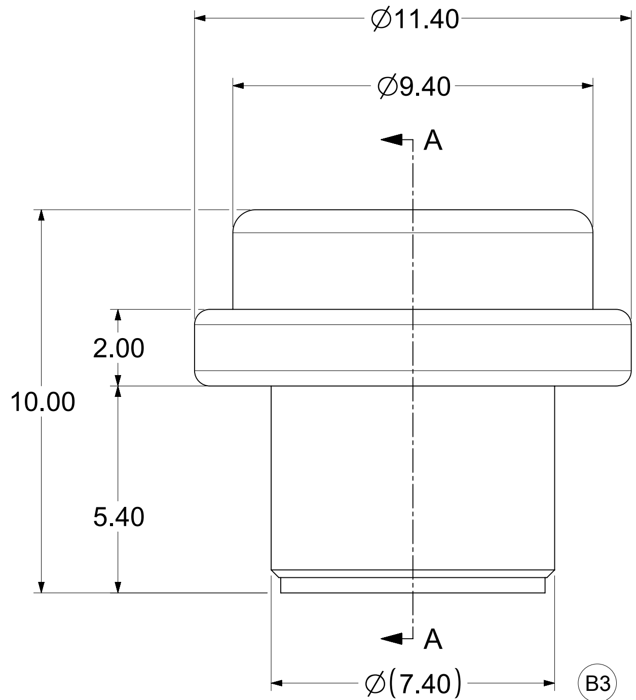
SOCKET ALONE
