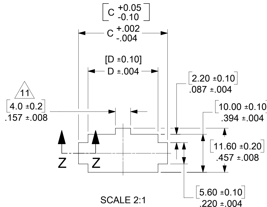
12 RECOMMENDED PANEL DIMENSIONS ( THICKNESS : 0.8-2.0/.032-.079 )
