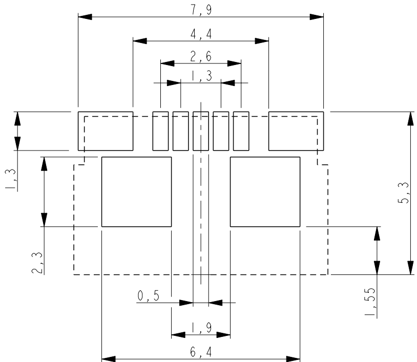
RECOMMENDED PWB LAYOUT
