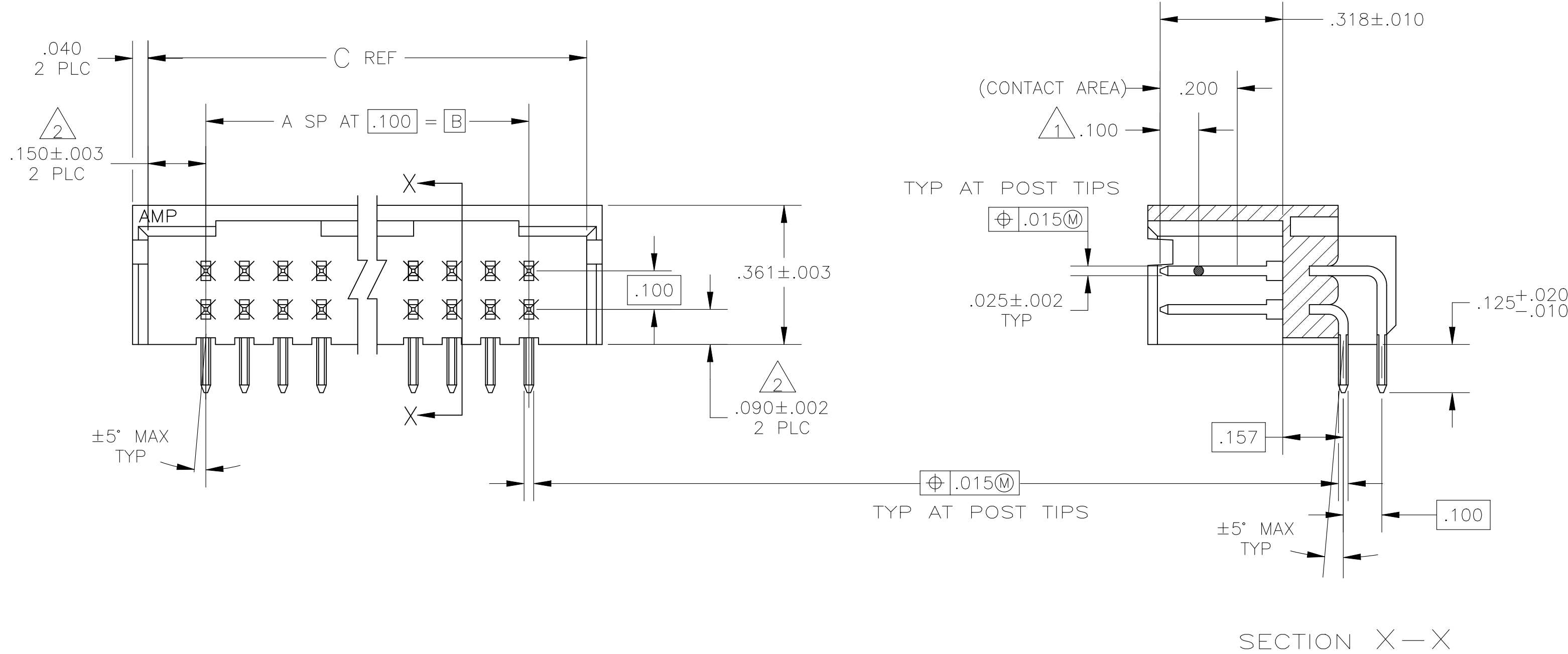
SECTION X-X
